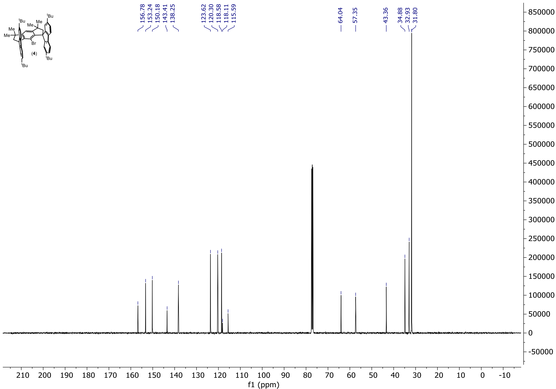
^{13}\text{C} NMR of t\text{Bu} -MsFluidBr ( 4 ) (101 MHz, \text{CDCl}_3 )
